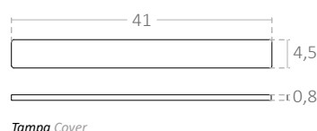
Tampa Cover
